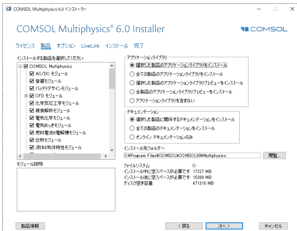
図3.1-4 “Products”画面
