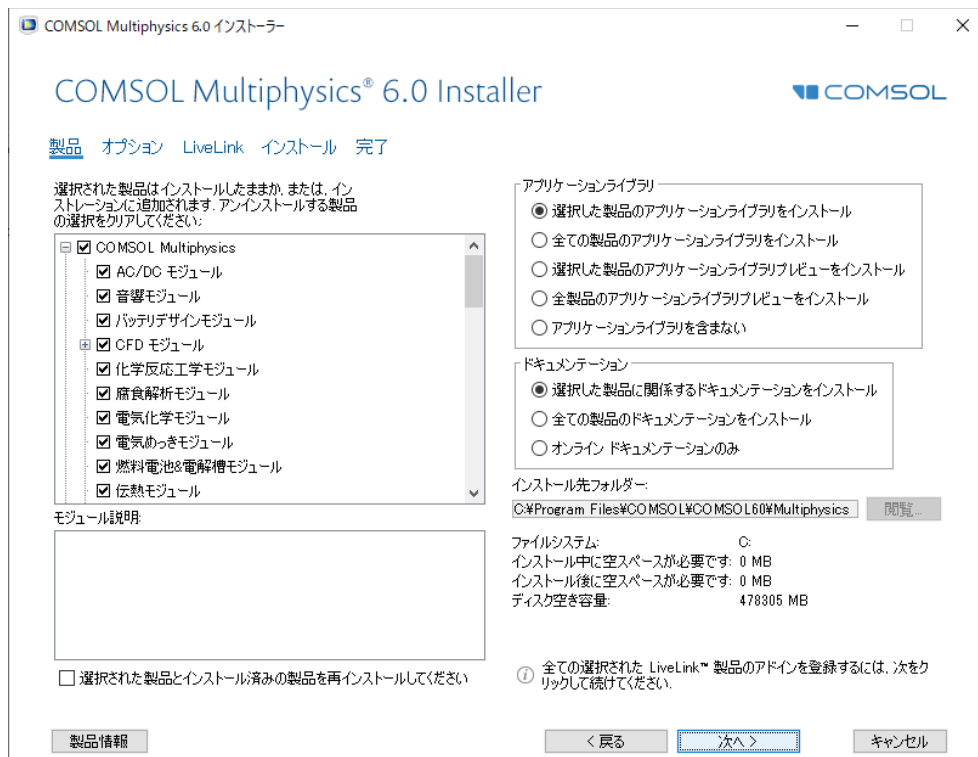
図4.3-3 “Products”画面
