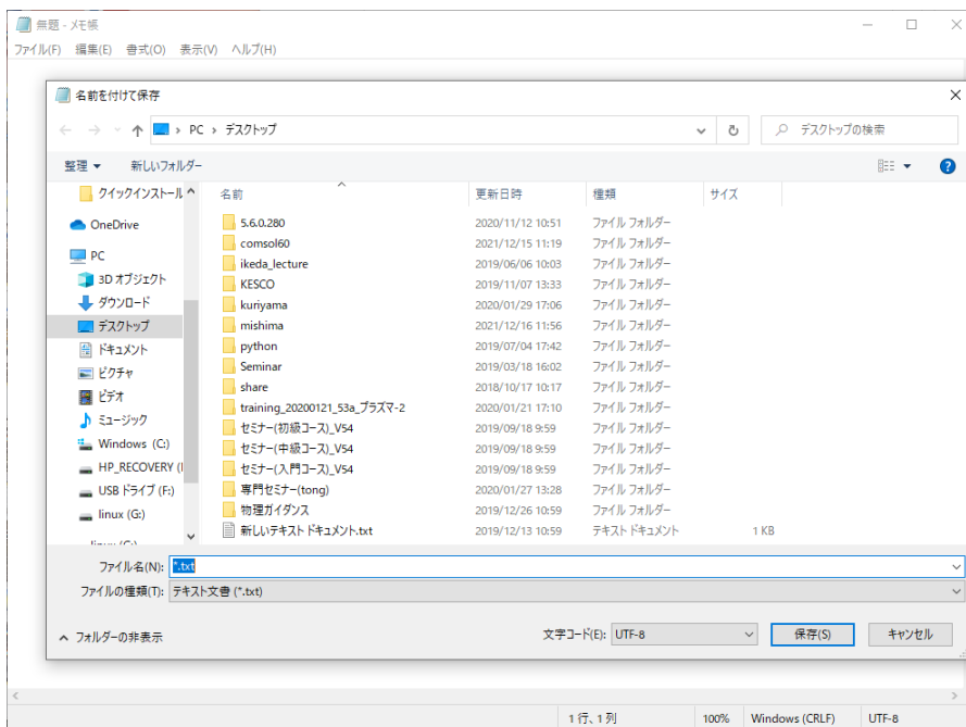
図2.3-3 comsol56.logの保存
