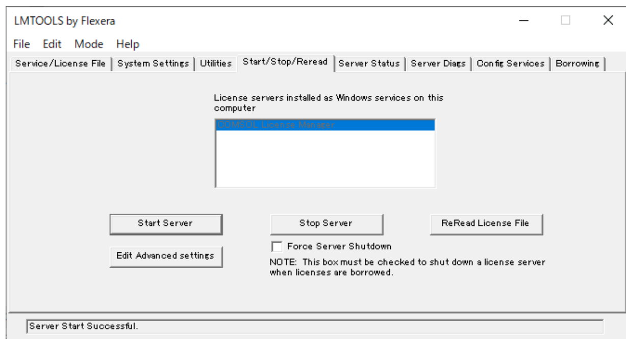
図2.3-10 “Start/Stop/Reread”画面
